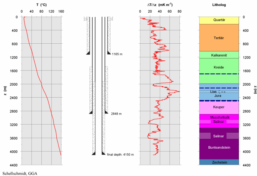
Figure 2: Depth profile of temperature, temperature gradient, stratigraphy and scheme of the well completion of the Horstberg Z1 well.
